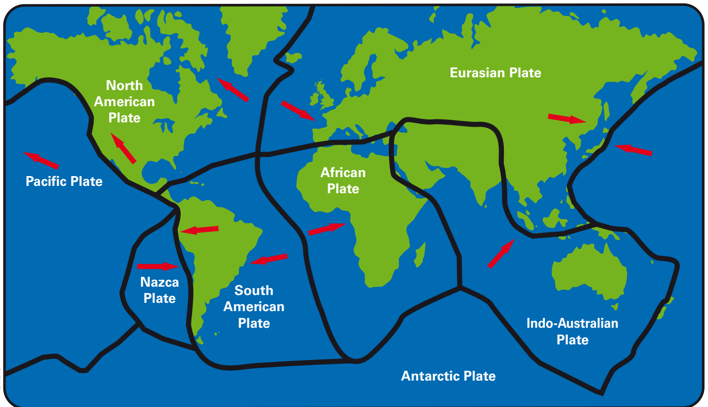
Simplified plate tectonics map of the world.
