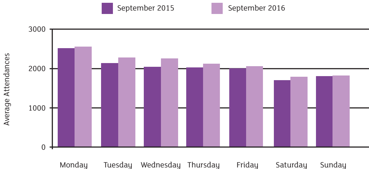
Average Number of Attendances at Emergency Care Departments by Day of Week (September 2015 and September 2016)
