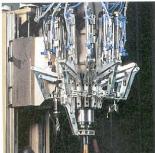
(a) Production line of CD-ROM (b) Mechanical clamp Fig. 2 Examples of pneumatic systems
