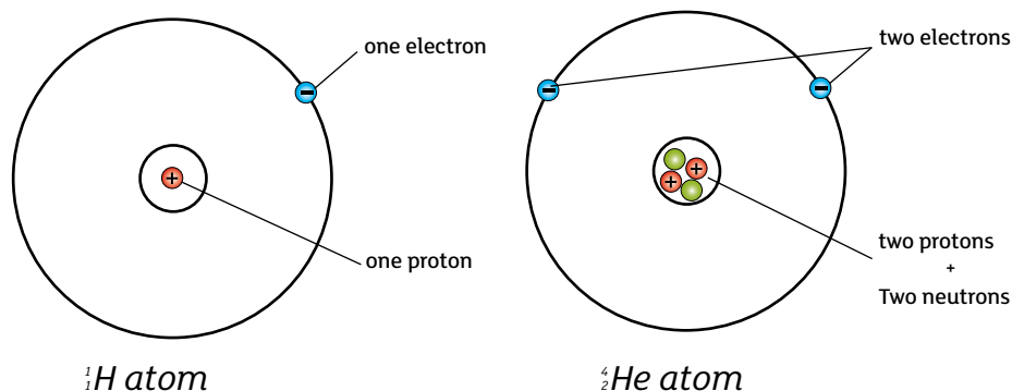
Atoms of {}^1_1\text{H} and {}^4_2\text{He}
